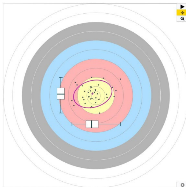
Figure 7: Boxplots
