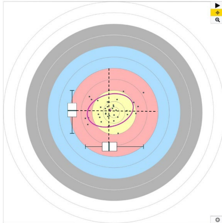
Figure 8: Median
