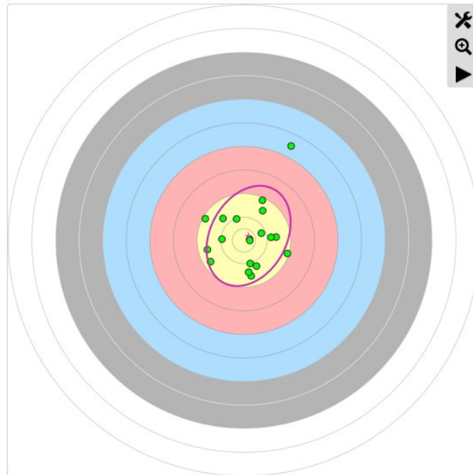
Figure 5: Effect of outliers
