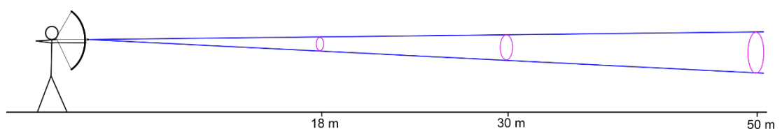
Figure 6: AGI and distance
