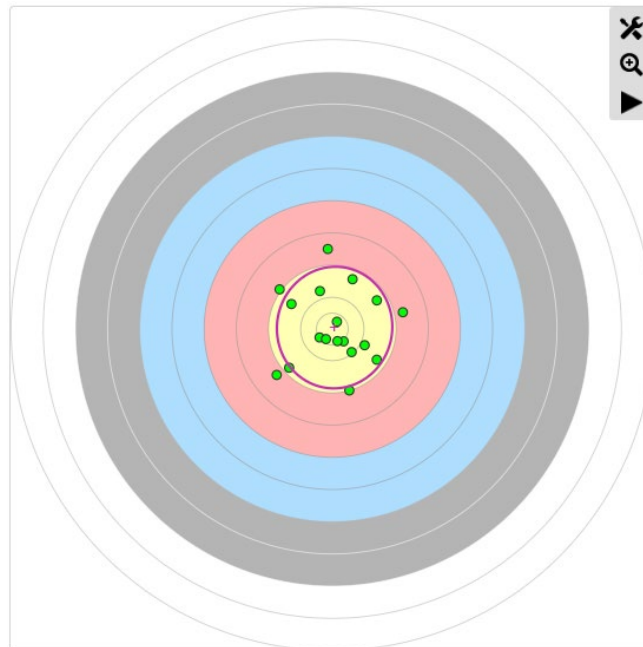
Figure 4: Scatter ellipse as a circle
