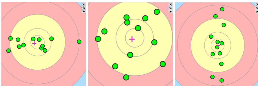
Figure 2: Same Group Center – Varying Dispersions
