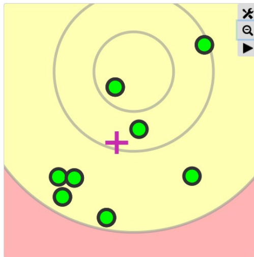
Figure 1: Group Center
