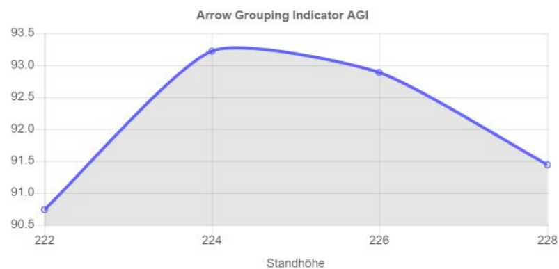
Figure 11: AGI – Brace height
