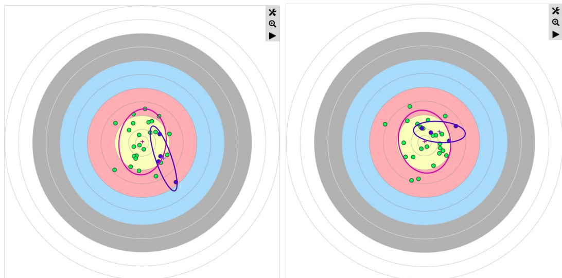
Figure 12: Bare Shaft Test for Nocking Point
