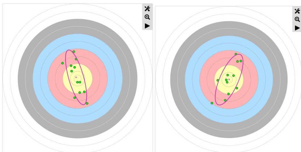
Figure 3: Rotated Scatter Ellipses
