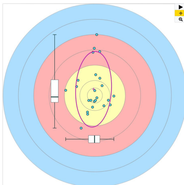
Figure 9: Vertically asymmetric hit distribution
