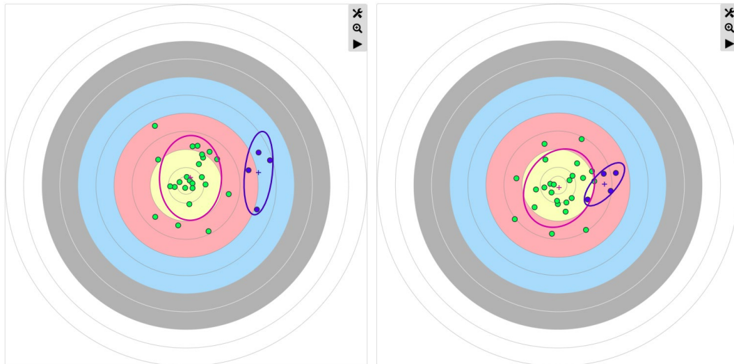
Figure 14: Bare Shaft Test for Arrow Length
